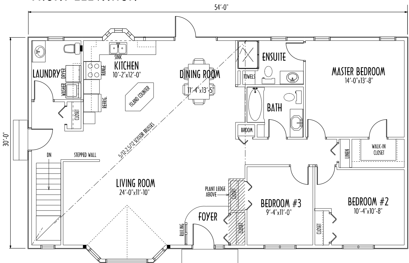
MAIN FLOOR PLAN AREA 1638 SQ.FT.
