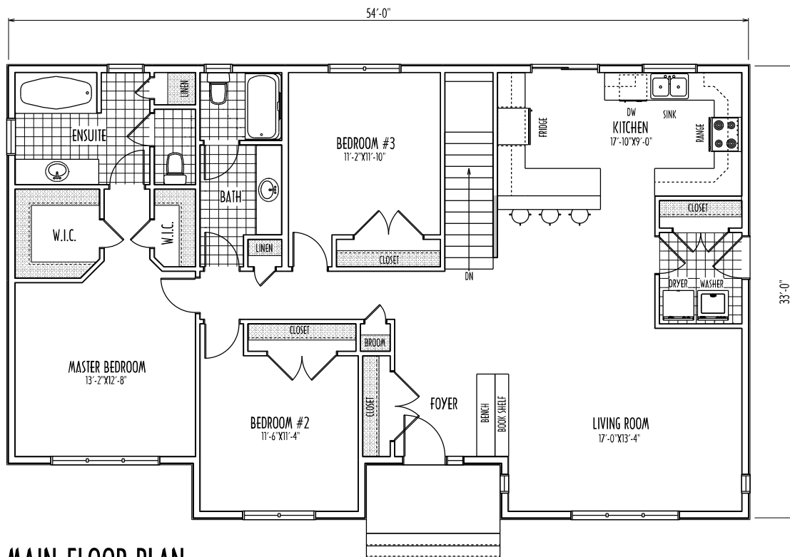
MAIN FLOOR PLAN AREA 1688 SQ.FT.
