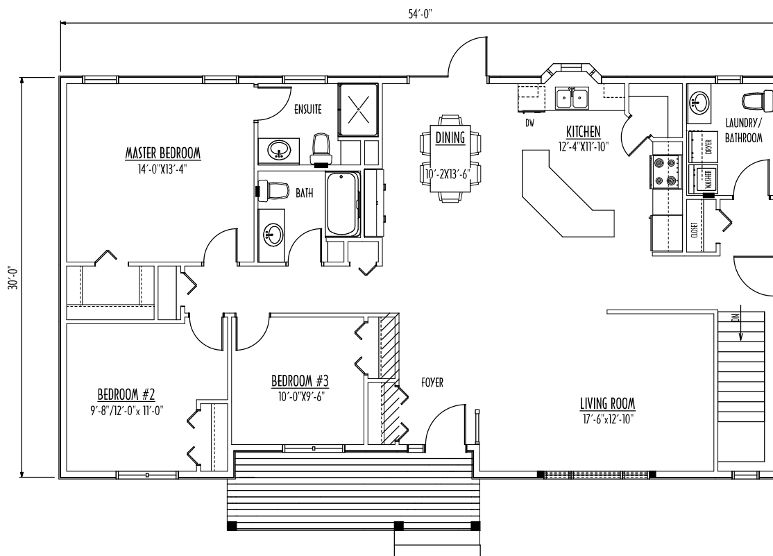
MAIN FLOOR PLAN AREA 1584 SQ.FT.
