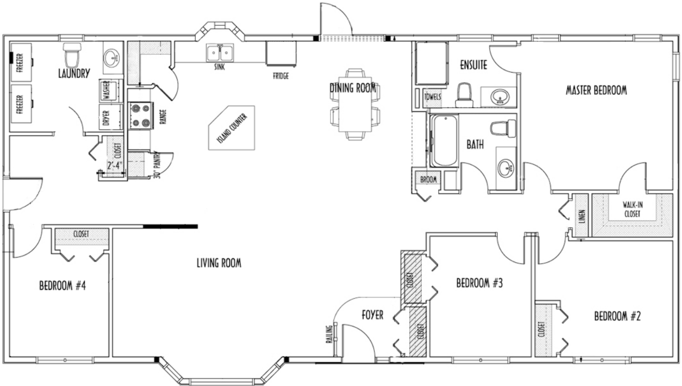
MAIN FLOOR PLAN AREA 1880 SQ.FT.
