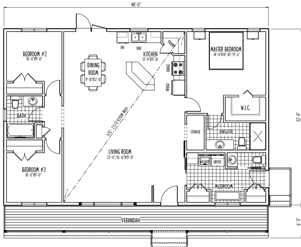
MAIN FLOOR PLAN AREA 1536 SQ.FT.
