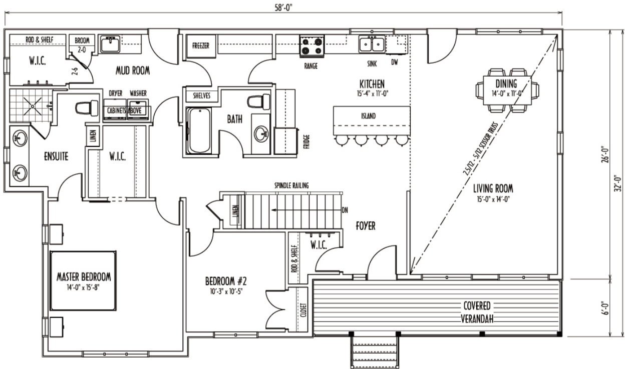
MAIN FLOOR PLAN AREA 1669 SQ. FT.
