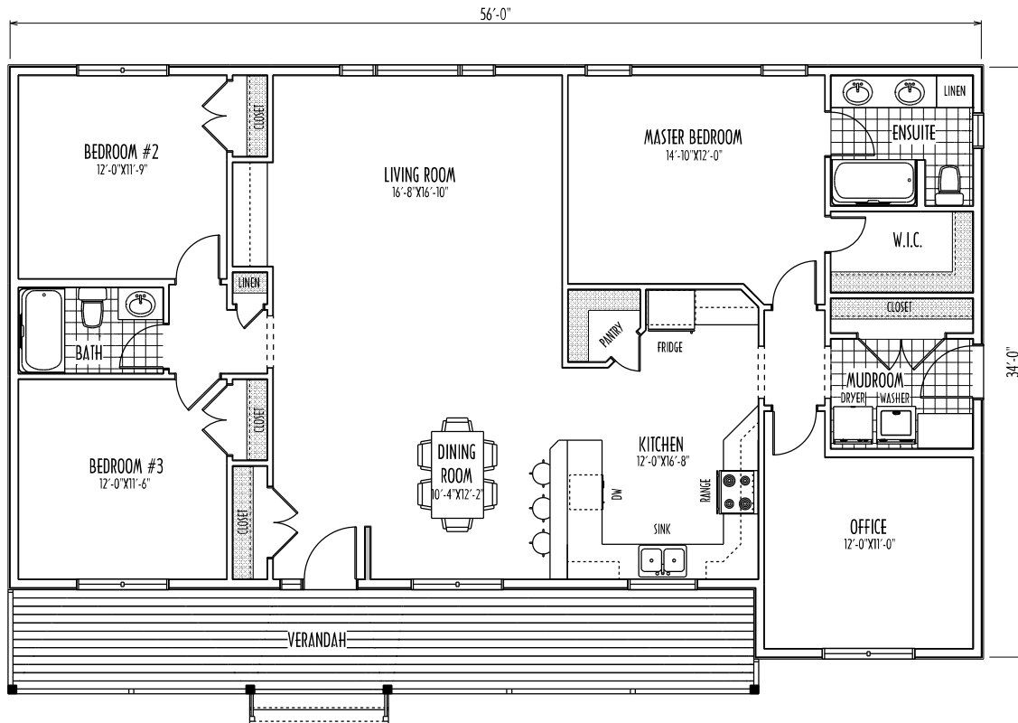
MAIN FLOOR PLAN AREA 1732 SQ.FT.
